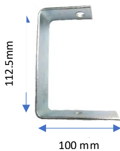
A-MAX 2"x4" Trunking Bracket 100mm(L) x 32mm(W) x 112.5mm(H) 2.8mm(thickness) x 32mm(W) flat bar
