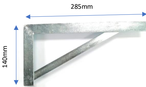
A-MAX 140mm x 285mm L Bracket (Heavy Duty) 285mm(L) x 24mm(W) x 140mm(H)
