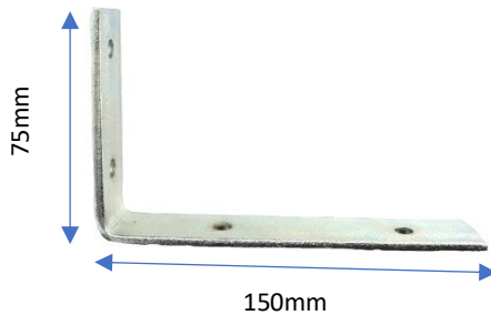
A-MAX 3"x6" L Bracket 150mm(L) x 24mm(W) x 75mm(H) 4.5mm(thickness) x 24mm(W) flat bar
