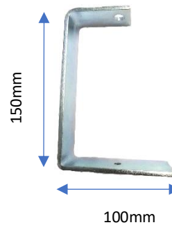
A-MAX 3"x4" / 4"x4" Trunking 100mm(L) x 32mm(W) x 150mm(H) 4.5mm(thickness) x 32mm(W) flat bar
