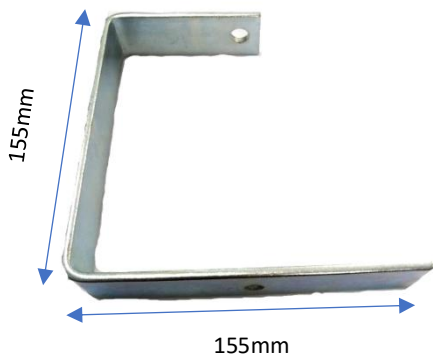
A-MAX 4"x6" Trunking Bracket 155mm(L) x 32mm(W) x 155mm(H) 4.5mm(thickness) x 32mm(W) flat bar
