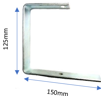
A-MAX 3"x6" Trunking Bracket (Eco) 150mm(L) x 25mm(W) x 125mm(H) 4.5mm(thickness) x 25mm(W) flat bar
