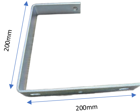
A-MAX 6"x8" Trunking Bracket 200mm(L) x 32mm(W) x 200mm(H) 4.5mm(thickness) x 32mm(W) flat bar
