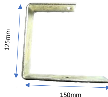
A-MAX 3"x6" Trunking Bracket (Premium) 150mm(L) x 32mm(W) x 125mm(H) 4.5mm(thickness) x 32mm(W) flat bar
