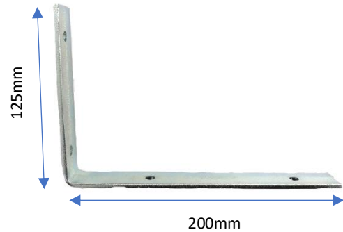
A-MAX 5"x8" L Bracket 200mm(L) x 25mm(W) x 125mm(H) 4.5mm(thickness) x 25mm(W) flat bar
