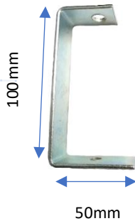
A-MAX 2"x2" Trunking Bracket 50mm(L) x 25mm(W) x 100mm(H) 2.8mm(thickness) x 25mm(W) flat bar
