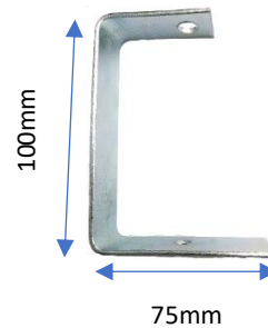
A-MAX 2"x3" Trunking Bracket 75mm(L) x 25mm(W) x 100mm(H) 2.8mm(thickness) x 25mm(W) flat bar
