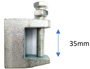
35mm Beam Clamp (Cast Iron) Weight : 270g
