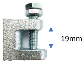
19mm Beam Clamp (Cast Iron) Weight : 140g
